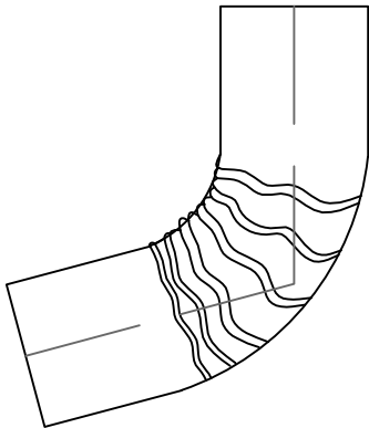
○ 75° ELBOW TYPE: #3
